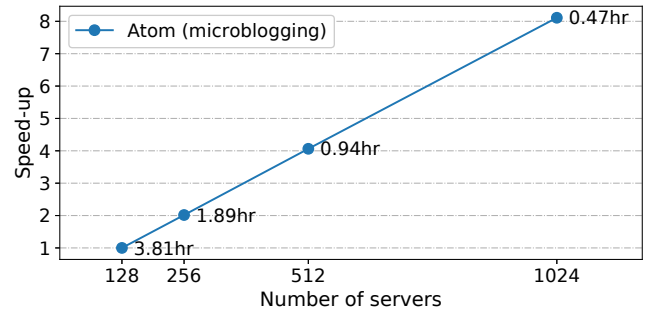
Figure 10. Speed-up of Atom networks of varying sizes relative to an Atom network of 128 servers. The speed-up is linear in the number of servers in the network.
