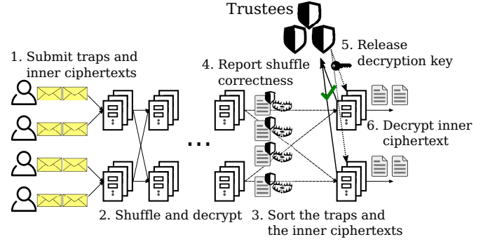
Figure 2. Atom with trap messages and trustees.
