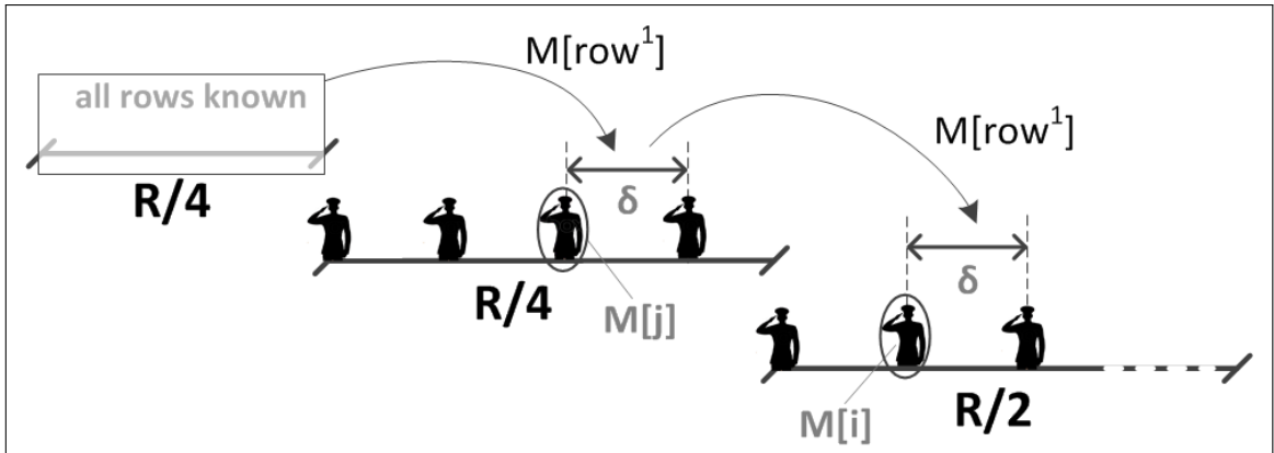
Figure R1: Low-memory attack using sentinels: against v1.
