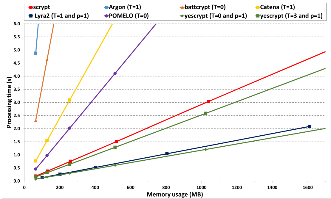
Figure 21: Performance of SSE-enabled Lyra2 with BlaMka G function, for C = 256 , \rho = 1 , p = 1 , and different T and R settings, compared with SSE-enabled script and memory-hard PHC finalists (configurations with a similar number of calls to the underlying function are marked with the same symbol, \blacksquare ).
