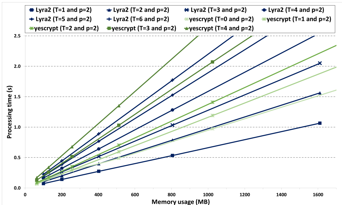
Figure 22: Performance of SSE-enabled Lyra2 with BlaMka G function, for C = 256 , \rho = 1 , p = 2 , and different T and R settings, compared with SSE-enabled yescript. Configurations with a similar number of calls to the underlying function are marked with the same symbol, \blacksquare or \blacktriangle .
