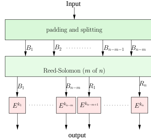
Fig. 2. AddRedundancy Operation
