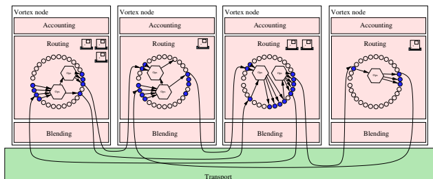
Figure 4.2: A generic overview for the protocol showing a circular path of a message
