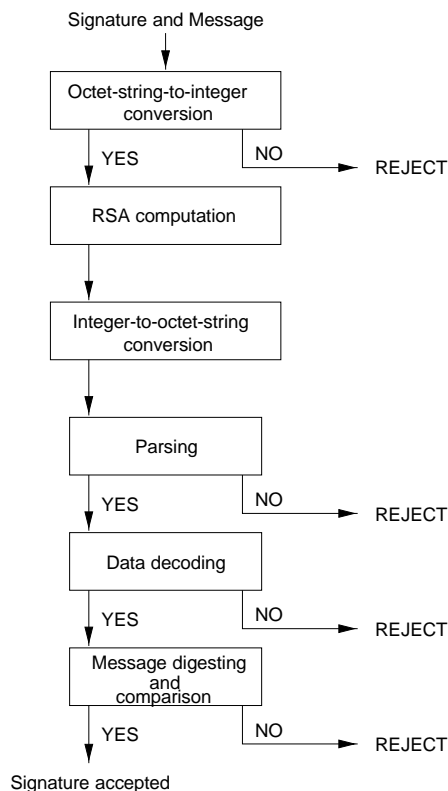
Figure 11.6: Signature and verification processes for PKCS #1.
